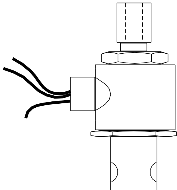
3-way solenoid valve - normally closed ( \frac{1}{8} " NPT)
